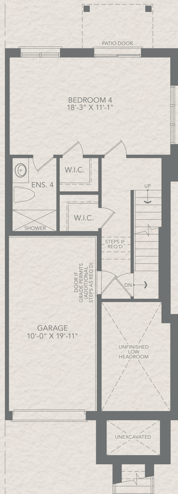
OPT. GROUND FLOOR PLAN EL. A1
