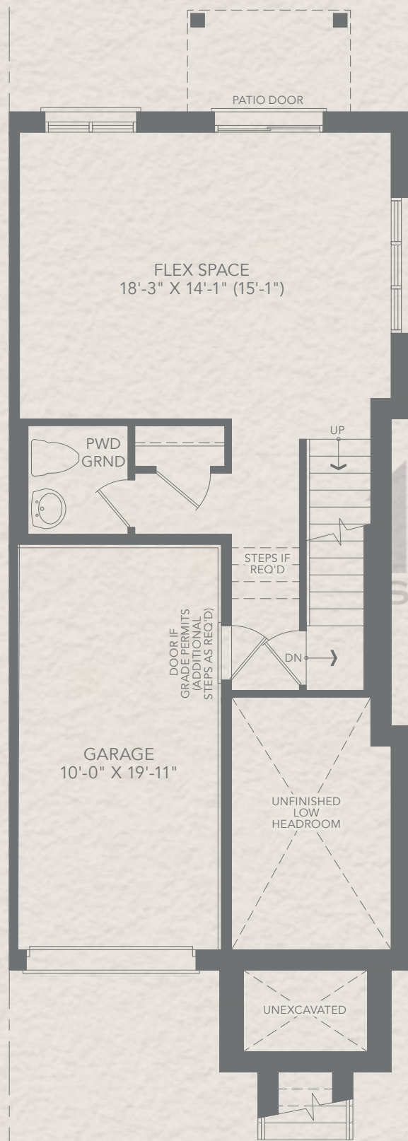
GROUND FLOOR PLAN EL. A1
